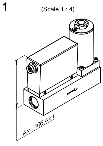
M+W analog case assy
